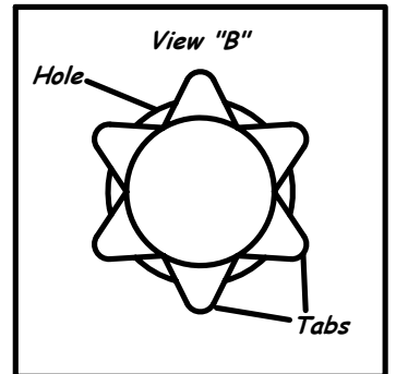
Underside of Fender Brace Cover
